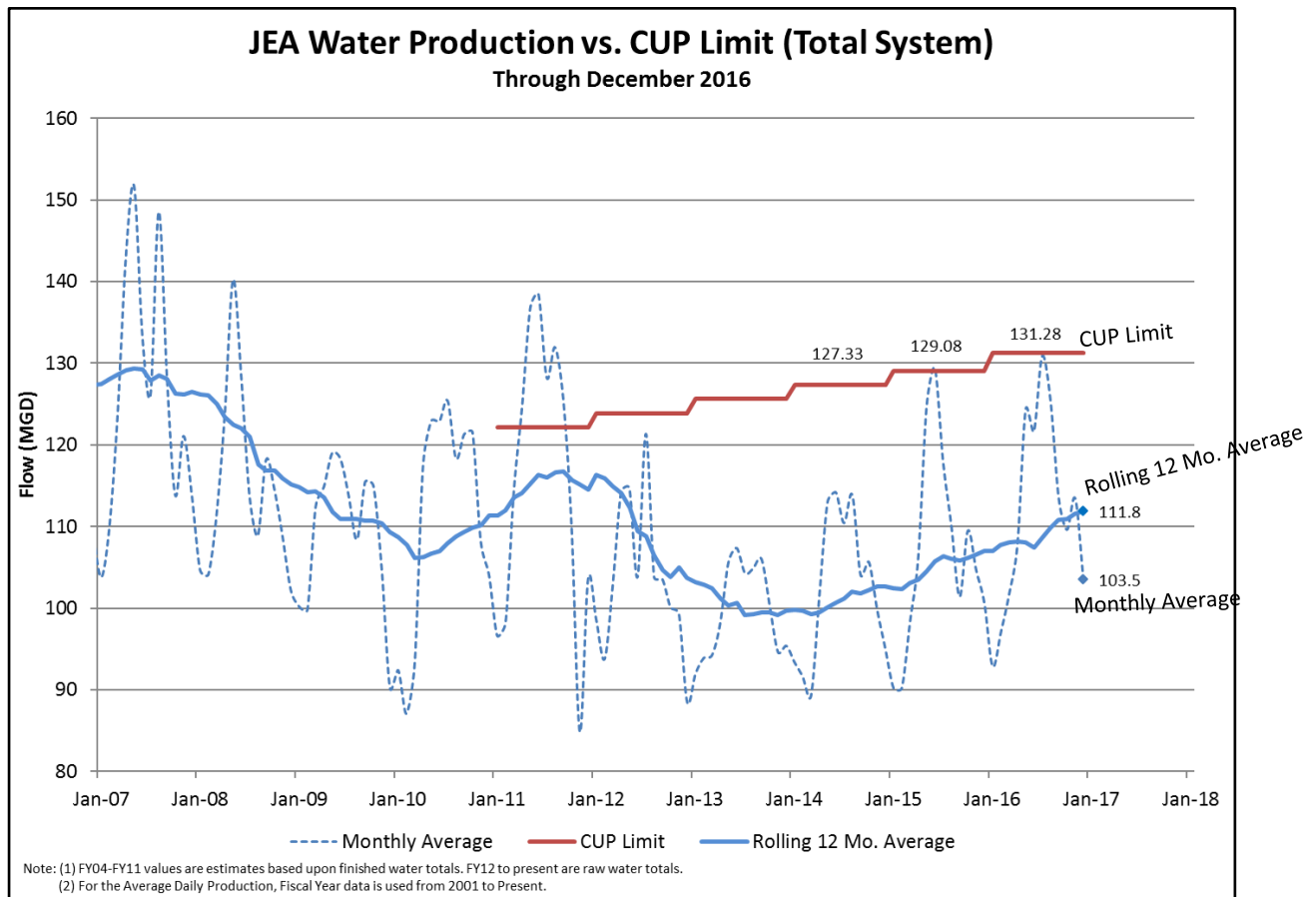
Figure 6: JEA Water Production vs. CUP Limit Source: JEA’s 2017 Annual Water Resource Master Plan
